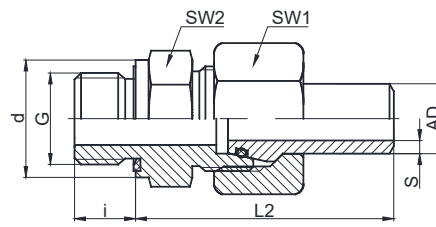
Weld Fitting
