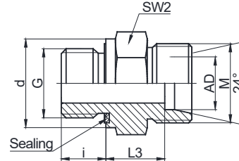
Body
