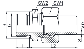
Weld Fitting
