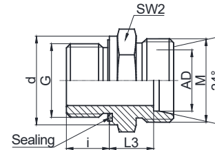
Body
