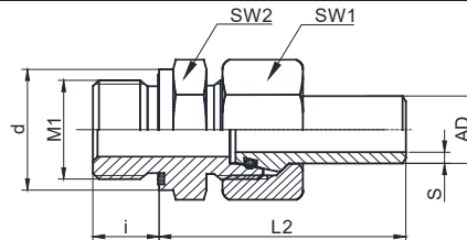
Weld Fitting
